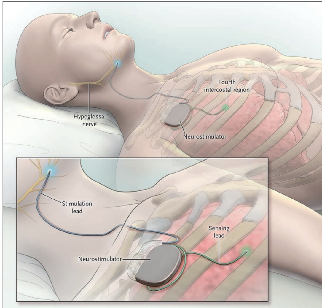
Figure 1. Upper-Airway Stimulation.
